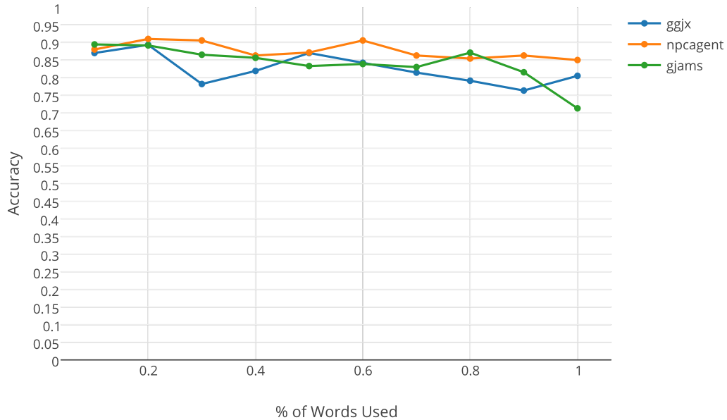
Figure 4.16: Accuracy of Entity Classification using Naive Bayes with a varying top word threshold.
