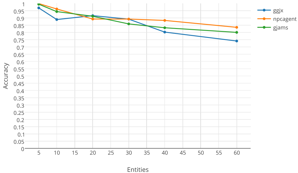
Figure 4.30: Accuracy of Entity Classification using Naive Bayes with a combined feature set of Taxonomy, Link, and BoW.
