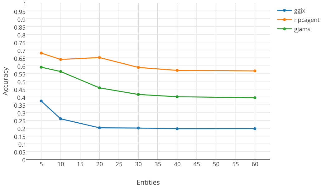
Figure 4.21: Accuracy of Megam classifier with the PoSTrigram feature set.
