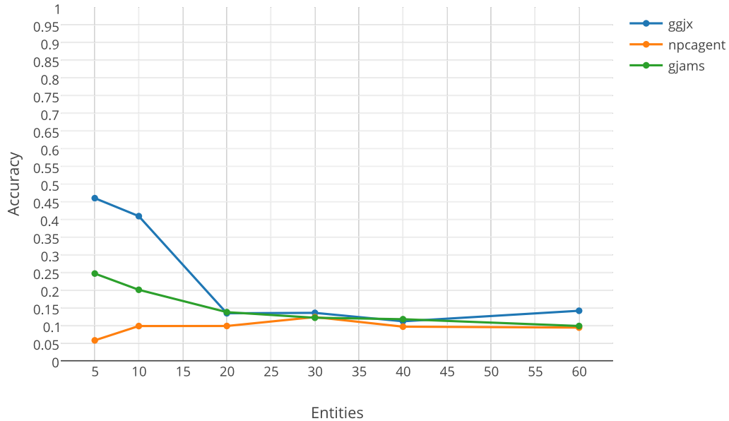
Figure 4.28: Accuracy of Entity Classification using Naive Bayes with the PoS Bigram feature set.
