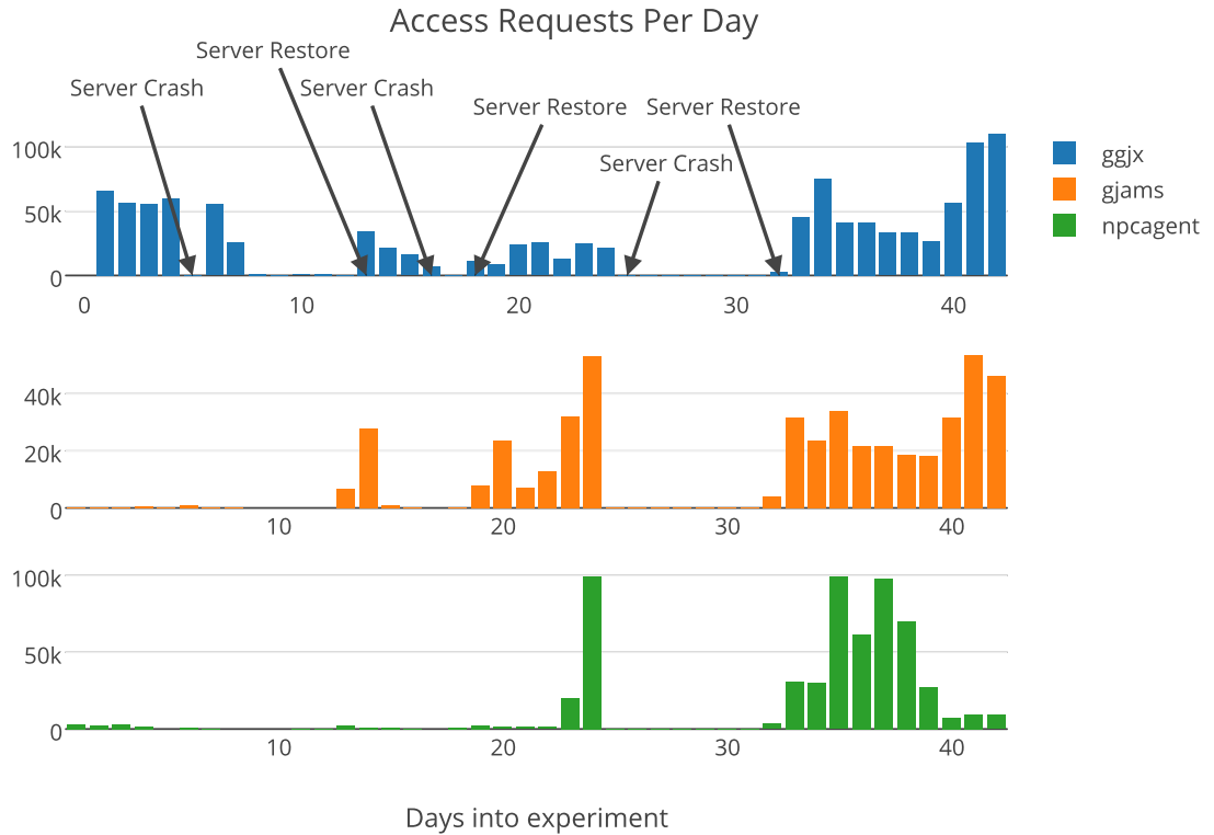
Figure 4.3: Access Requests Per Day.
