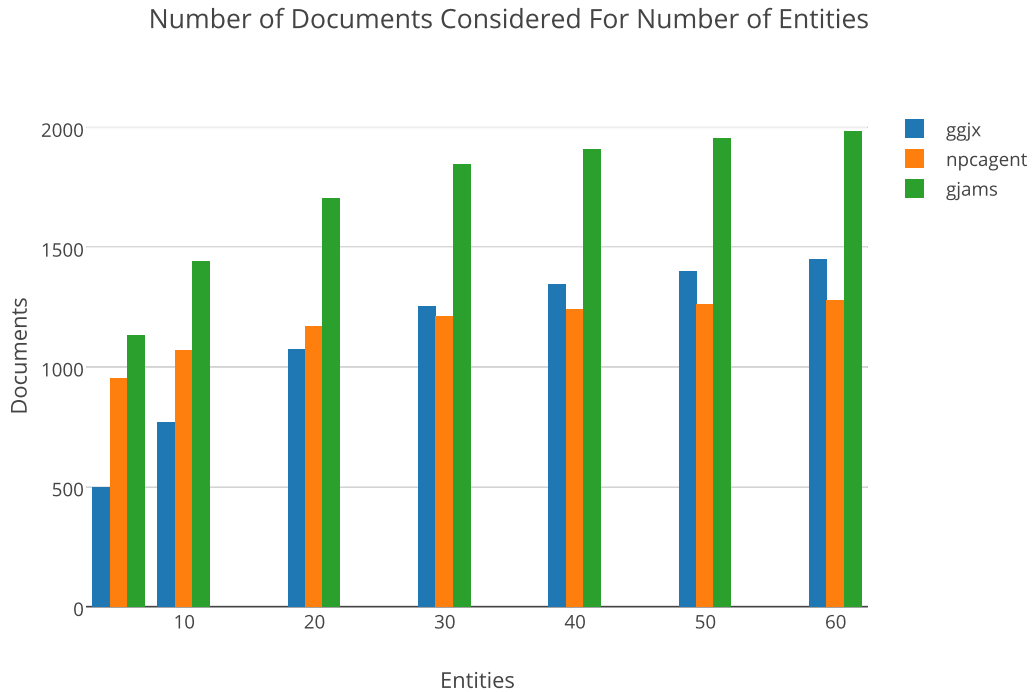
Figure 4.11: Number of Documents per Group of Entities.
