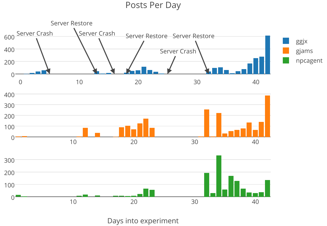
Figure 4.7: Posts Per Day.
