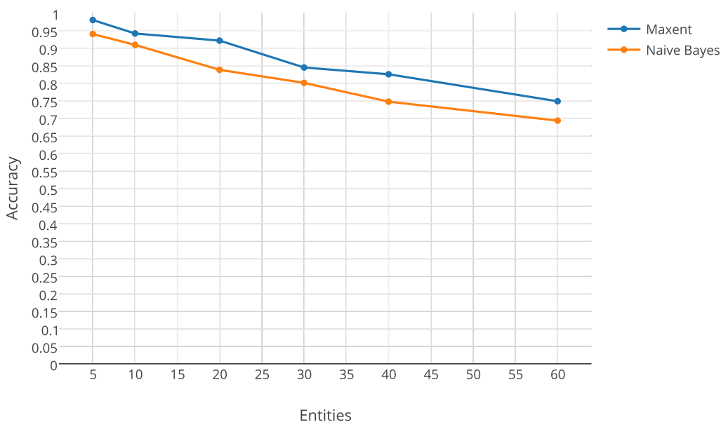
Figure 4.12: Prediction Accuracy With the Boolean feature set modification.
