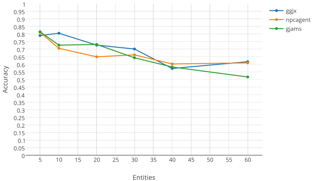
Figure 4.26: Accuracy of Naive Bayes classifier with the Alchemy Taxonomy feature set.
