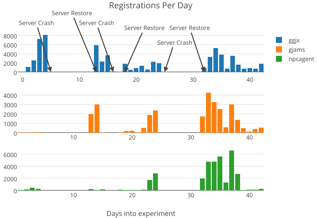
Figure 4.2: Registrations Per Day.
