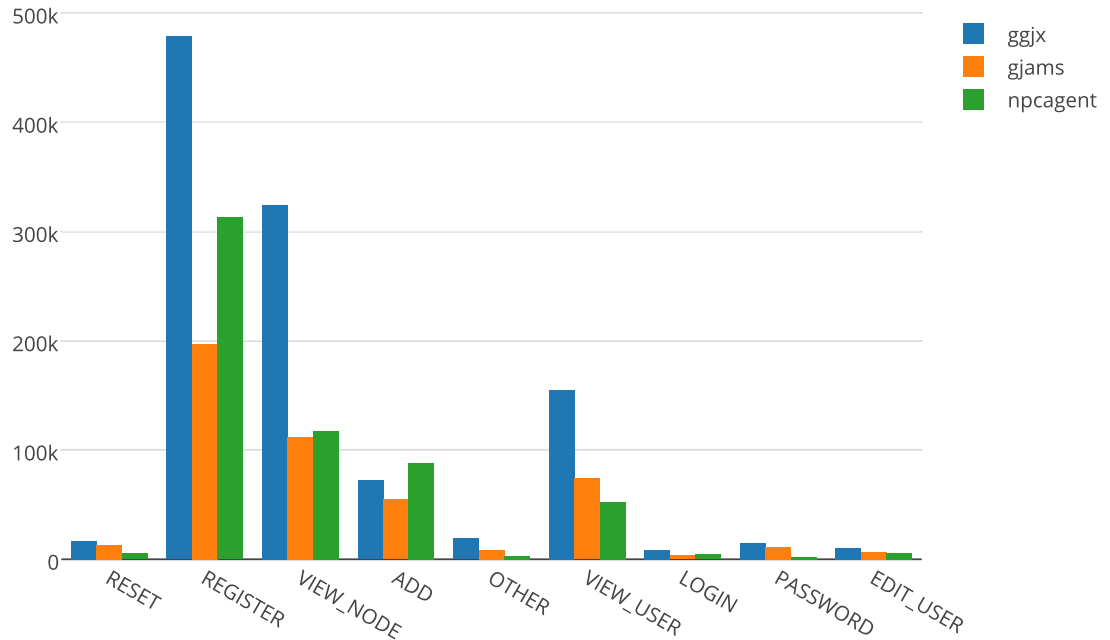
Figure 4.4: 'Action' type distribution.
