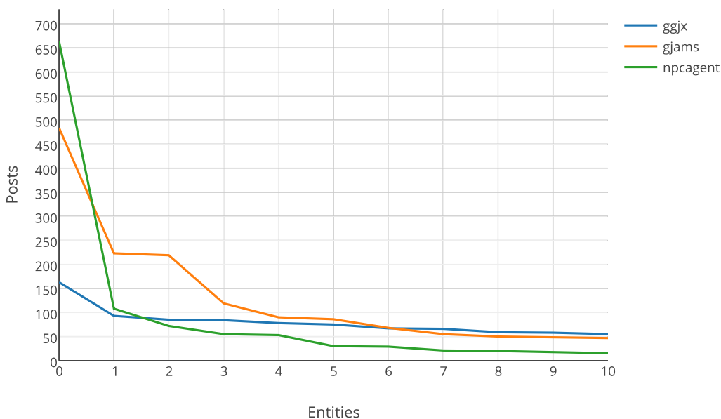
Figure 4.8: Post Frequency Distribution.
