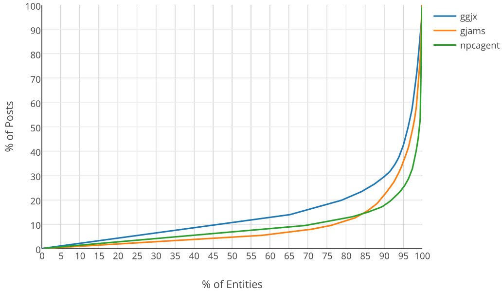
Figure 4.9: Cumulative Post Distribution when considering only entities who posted at least once.
