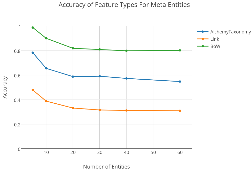
Figure 4.38: The accuracy of feature types with an isolated test set.
