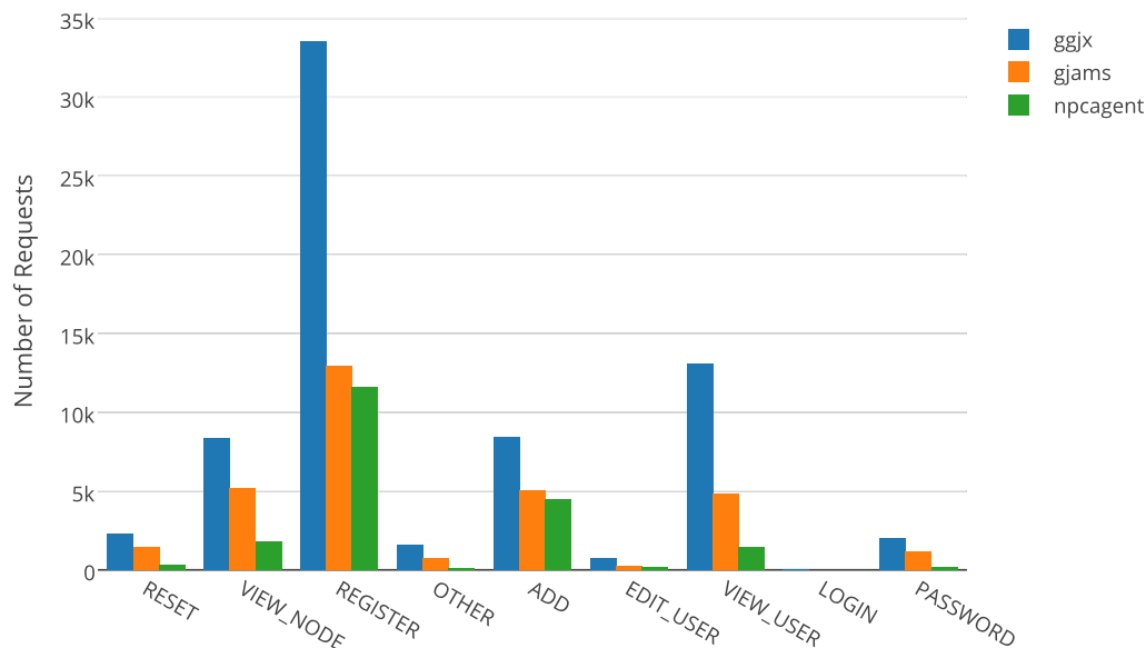
Figure 4.34: Access Requests for Scout IPs
