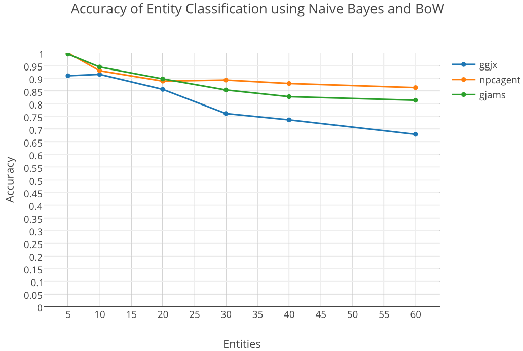
Figure 4.25: Accuracy of Naive Bayes classifier with the BoW feature set.
