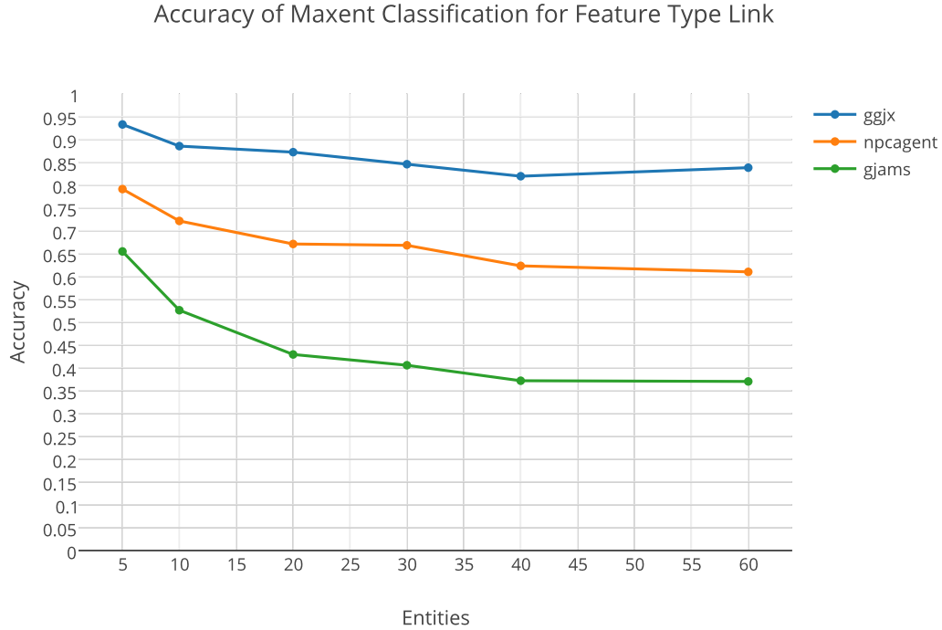
Figure 4.19: Accuracy of Megam classifier with the Link feature set.
