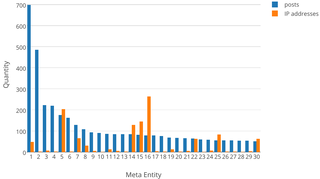
Figure 4.36: The meta entities’ post distribution compared to IP address distribution.
