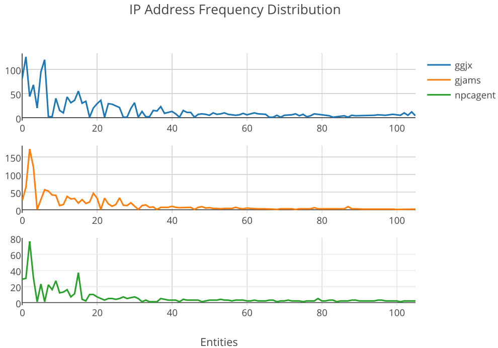
Figure 4.10: IP Frequency Distribution.
