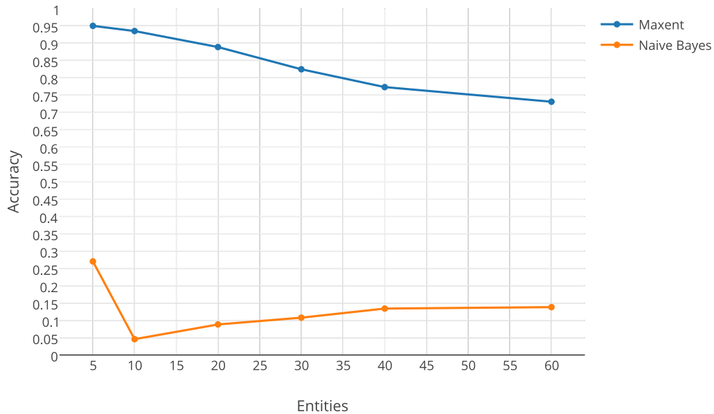
Figure 4.13: Prediction Accuracy With the normalization feature set modification.
