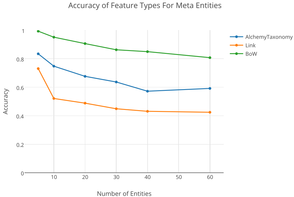
Figure 4.37: The accuracy of feature types with a collective feature set.
