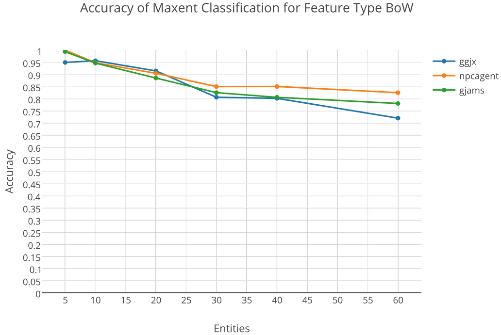
Figure 4.17: Accuracy of Megam classifier with the BoW feature set.
