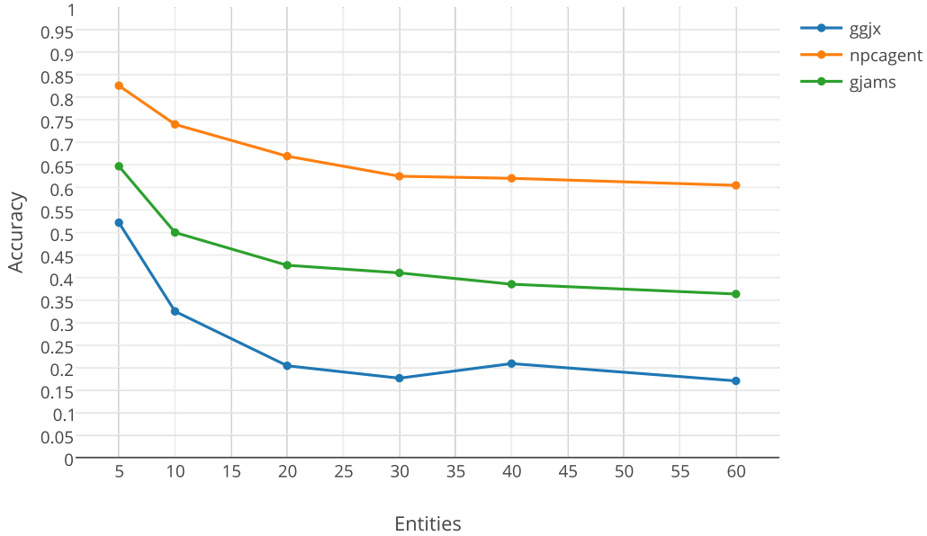
Figure 4.22: Accuracy of Megam classifier with the Vocab feature set.
