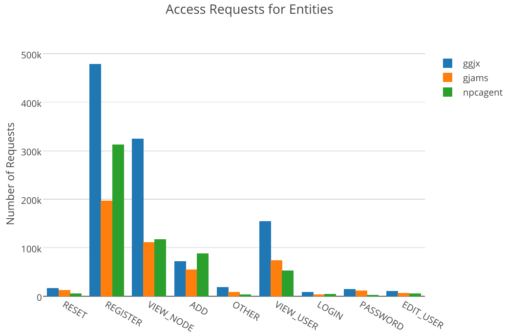
Figure 4.32: The ‘action’ category of access requests for entities.
