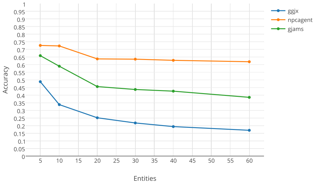
Figure 4.20: Accuracy of Megam classifier with the PoSBigram feature set.
