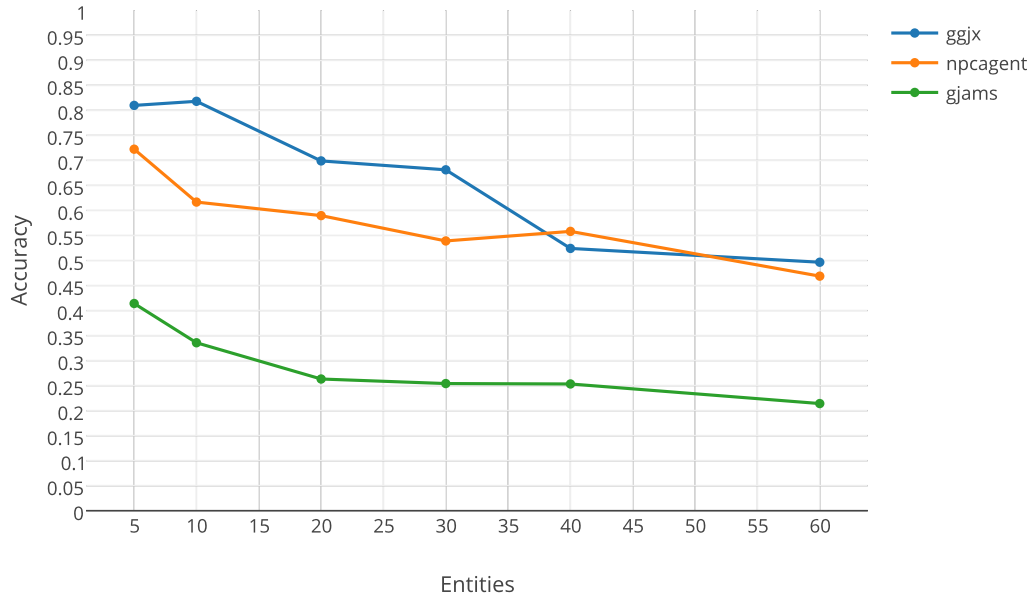
Figure 4.27: Accuracy of Naive Bayes classifier with the Link feature set.
