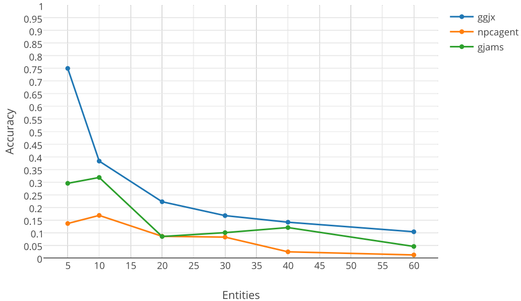
Figure 4.29: Accuracy of Entity Classification using Naive Bayes with the PoS Trigram feature set.
