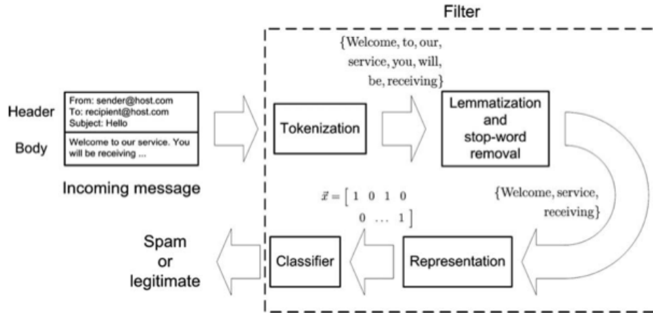
Figure 2.1: The Main Steps Involved in a Spam Filter [11].
