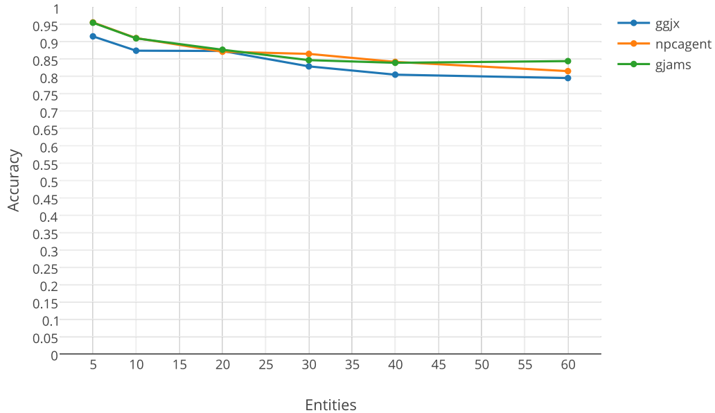
Figure 4.18: Accuracy of Megam classifier with the Alchemy Taxonomy feature set.
