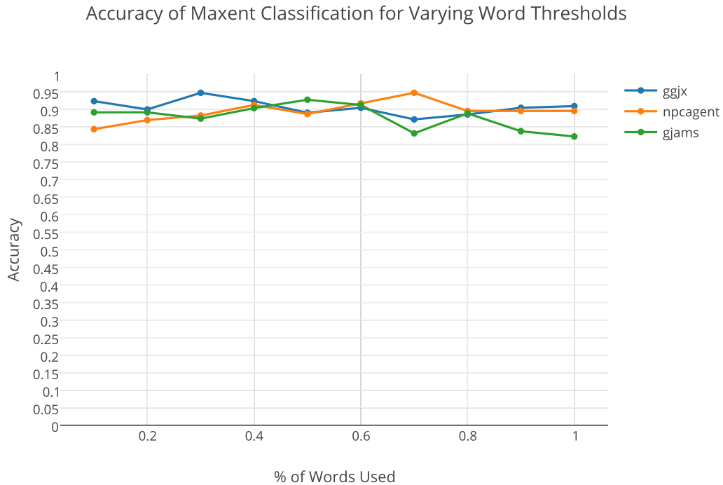
Figure 4.15: Accuracy of Megam classifier with a varying top word Threshold.
