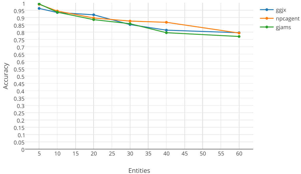
Figure 4.23: Accuracy of Megam classifier with the Taxonomy, BoW, and Link feature set.
