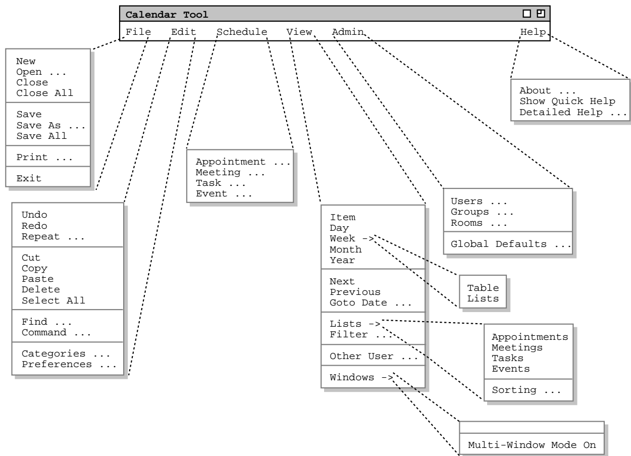
Figure 2: Expanded command menus.
