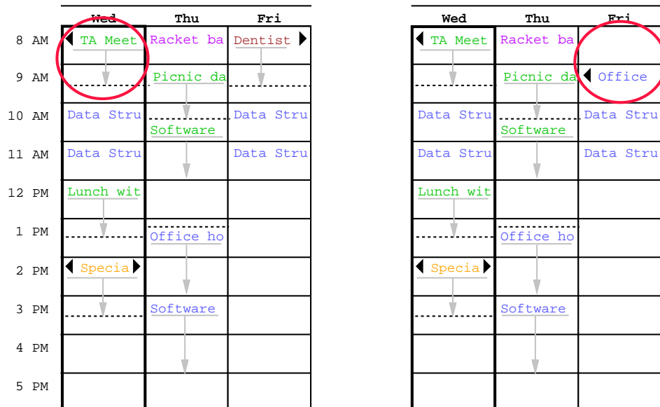
c. Pressed right arrow at Wed 8 AM.
