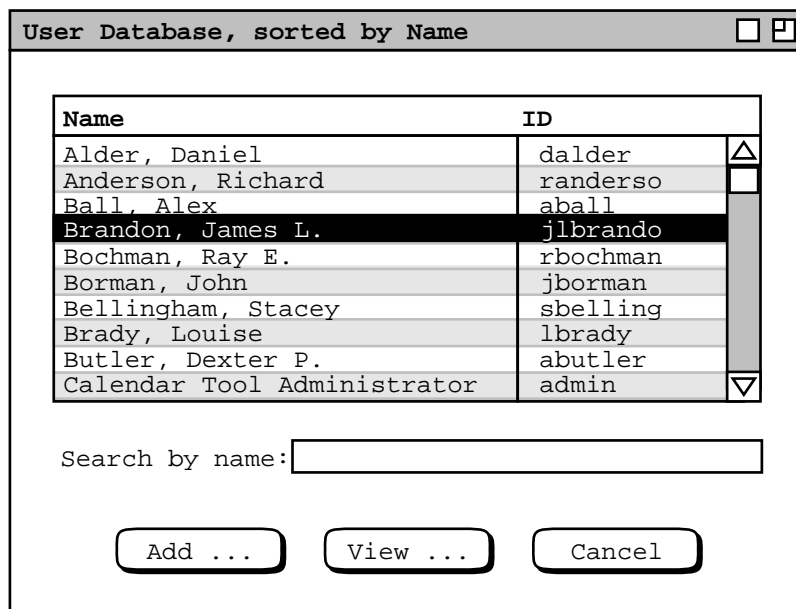
Figure 121: Brandon selected in users list.
