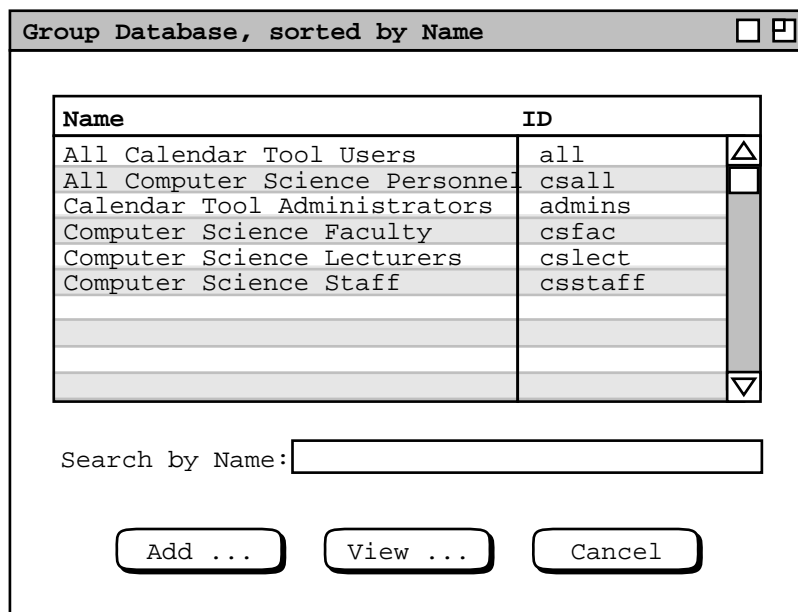
Figure 128: Group database dialog.
