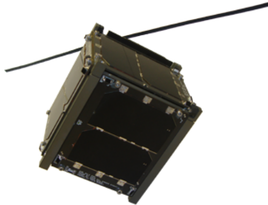
Figure 1.1: CP6, Cal Poly's Forth CubeSat
