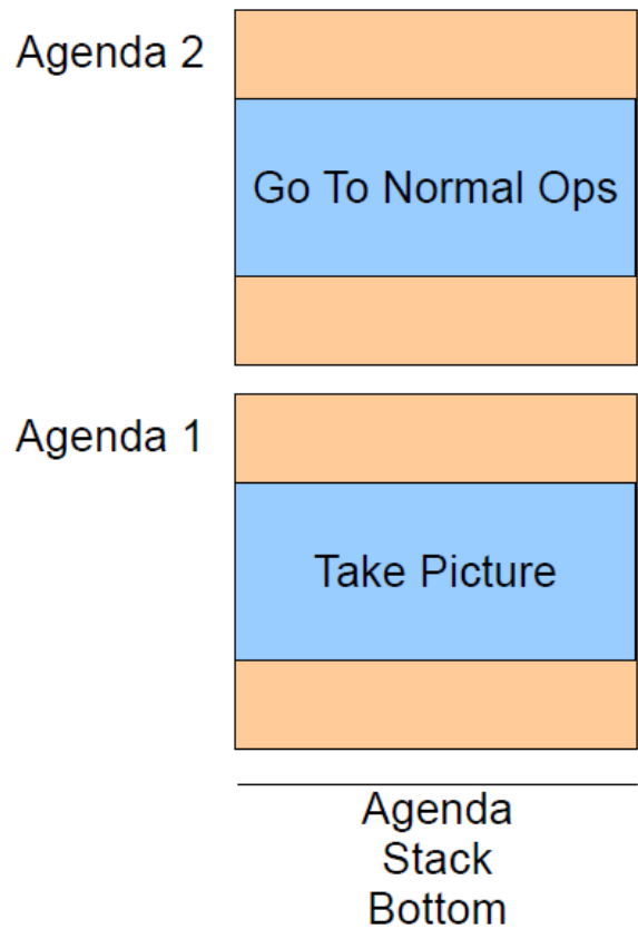
Figure 4.5: Agenda Stack after a Nack, Not in Normal Ops is Received
