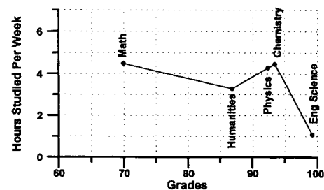
FIG. 5. Hours Studied versus Grades Illustrating a Potential Problem
