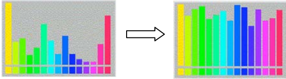
Figure 3 - Histogram equalization
