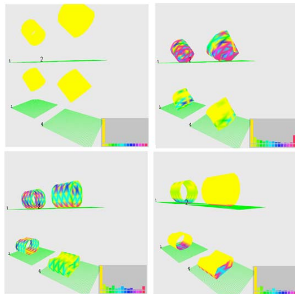
Figure 8 - The progression of forces in four dropped cylinders with varying internal force contributions.
