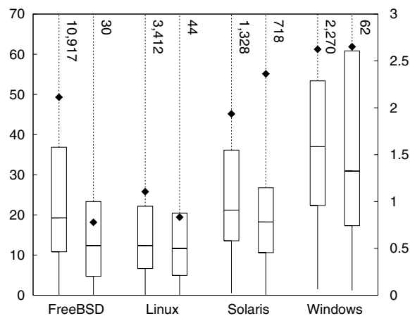
Figure 8: Comment density in C and header files.
