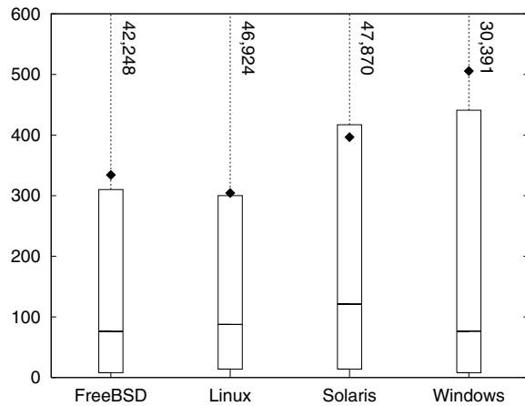
Figure 5: Halstead complexity.
